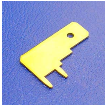
30-322 Tab: 6.35x0.8 Dimensions mm W: 7.7 Dimensions mm L: 20.0 Material: Brass
